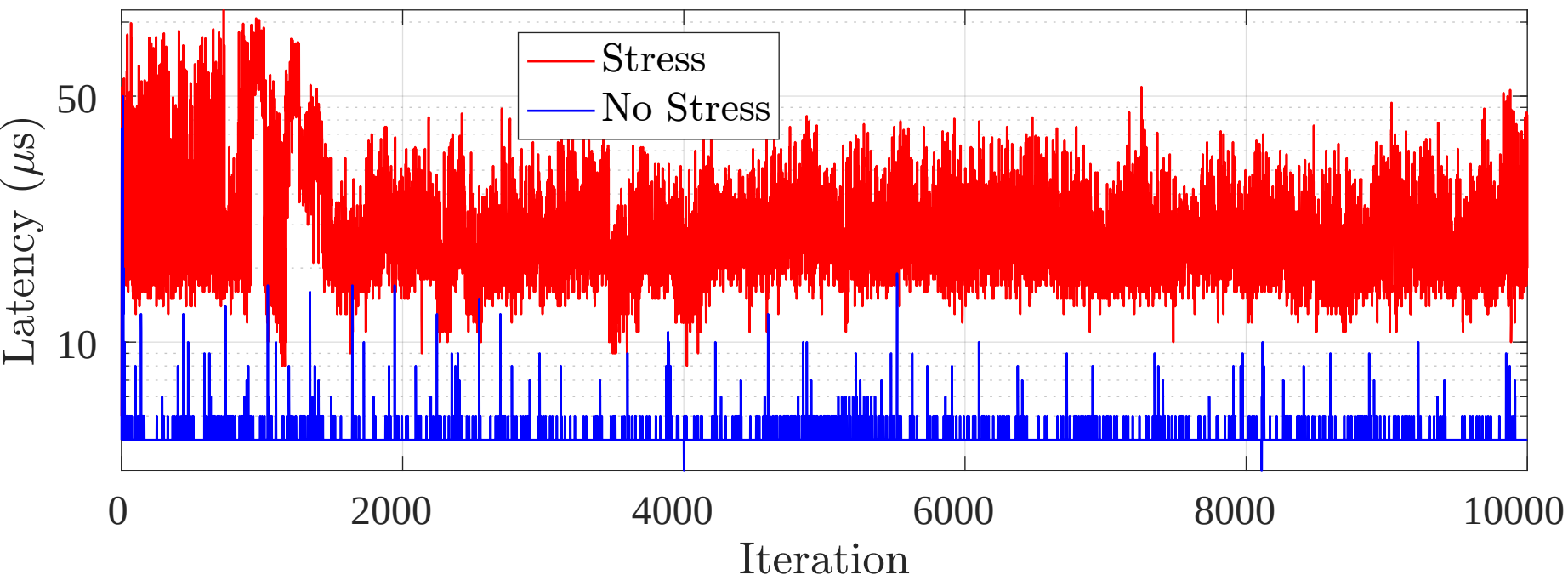
Latency for Scheduler: SCHED_FIFO p99
